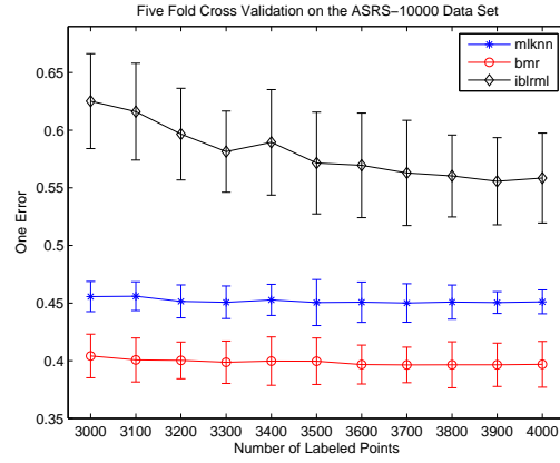
(b) One Error
