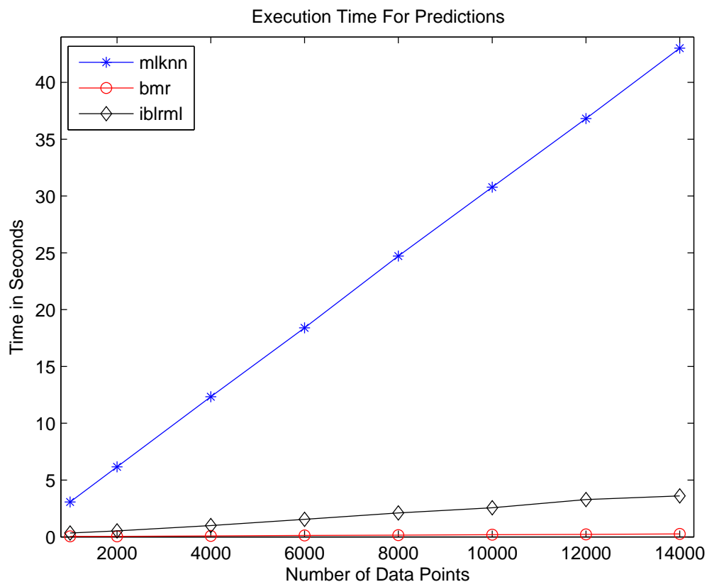
FIGURE 6. Computational time to make predictions as more and more points are considered. MBR outperforms MLKNN and IBLRML.
