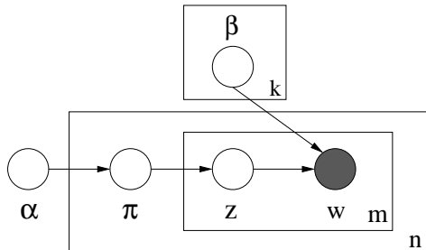
FIGURE 1. Graphical model for Latent Dirichlet Allocation.
