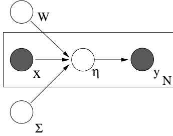
FIGURE 2. Graphical model for Bayesian Multivariate Regression.
