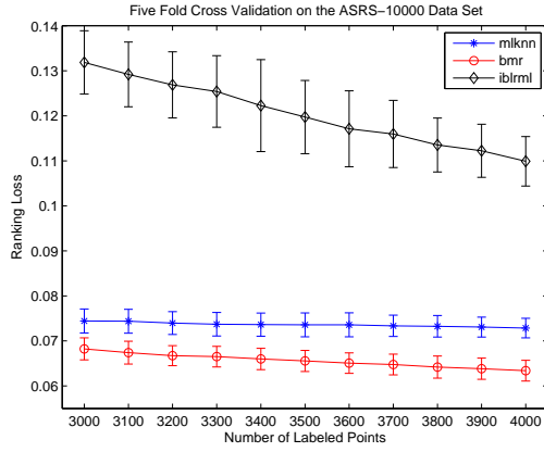
(a) Ranking Loss
