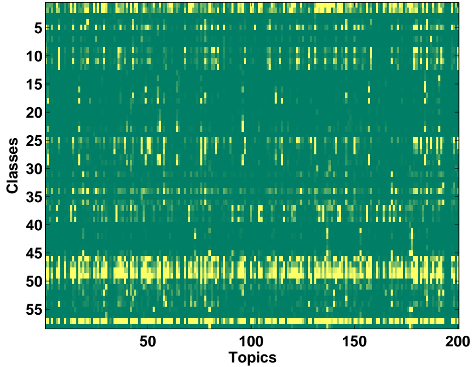
FIGURE 4. The relationship among 58 classes and 200 topics. A lighter color indicates a closer relationship.
