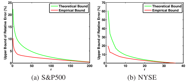
Figure 3: The upper bound of the relative error of the CCA results w.r.t. the global maximum on S&P 500 and NYSE in different dimensions r . The theoretical bound in (14) and empirical bound in (15) are in green and red, respectively. The upper bounds are very small for the first r principal components.
