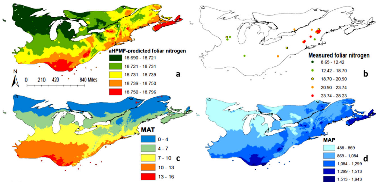
Figure 7 Advanced hierarchical probabilistic matrix factorization (aHPMF)-predicted leaf nitrogen concentration ( \text{mg g}^{-1} ) of Acer saccharum (a), measured values for leaf nitrogen ( \text{mg g}^{-1} ) (b), MAT (mean annual temperature) (c), and MAP (mean annual precipitation) (d) across the species range of A. saccharum . For a map of the geographic location see Figure S5.1 in Appendix S5.
