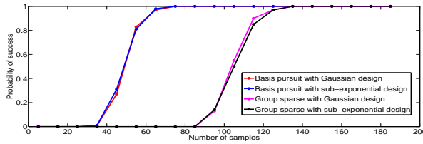
Figure 1: Probability of recovery in noiseless case with increasing sample size. There is a sharp phase transition and the curves overlap for Gaussian and sub-exponential designs.
