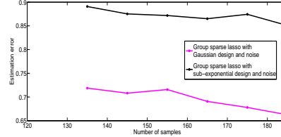
Figure 2: Estimation error \|\hat{\Delta}_n\|_2 vs sample size for \ell_1 (left) and group-sparse norms (right). The curve for sub-exponential designs and noise decays slower than Gaussians.
