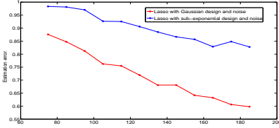
Figure 2: Estimation error \|\hat{\Delta}_n\|_2 vs sample size for \ell_1 (left) and group-sparse norms (right). The curve for sub-exponential designs and noise decays slower than Gaussians.
